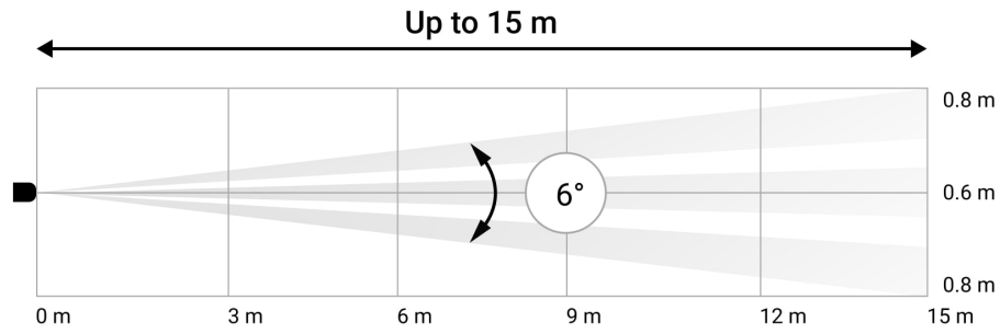
Horizontal and vertical detector's angles of view
